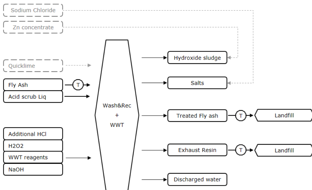
Figure 3. Scenario Wash&Rec, with Fluwa technology. Materials flows are represented with squares, while processes with hexagons. Round figures represent transportation processes, which expected distance has been part of the scenarios analysis. Dashed lines indicates the avoided production of virgin raw materials. [T: transportation; WWT: wastewater treatment]
