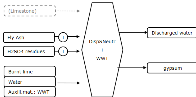
Figure 1. Scenario Disp&Neutr, with NOAH process. Materials flows are represented with squares, while processes with hexagons. Round figures represent transportation processes, which expected distance has been part of the scenarios analysis. Dashed lines indicates the avoided production of virgin raw materials. [T: transportation; WWT: wastewater treatment]
