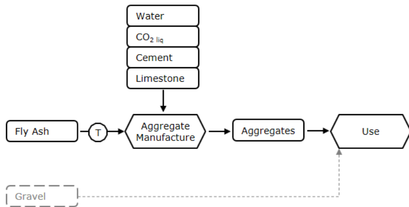
Figure 2. Scenario Aggregate, with Carbon8 Aggregates Ltd technology. Materials flows are represented with squares, while processes with hexagons. Round figures represent transportation processes, which expected distance has been part of the scenarios analysis. Dashed lines indicates the avoided production of virgin raw materials. [T: transportation]
